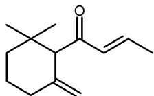
2-Buten-1-one, 1-(2,2-dimethyl-6-methylenecyclohexyl)-
